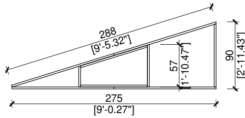
TRUSS FRAME
